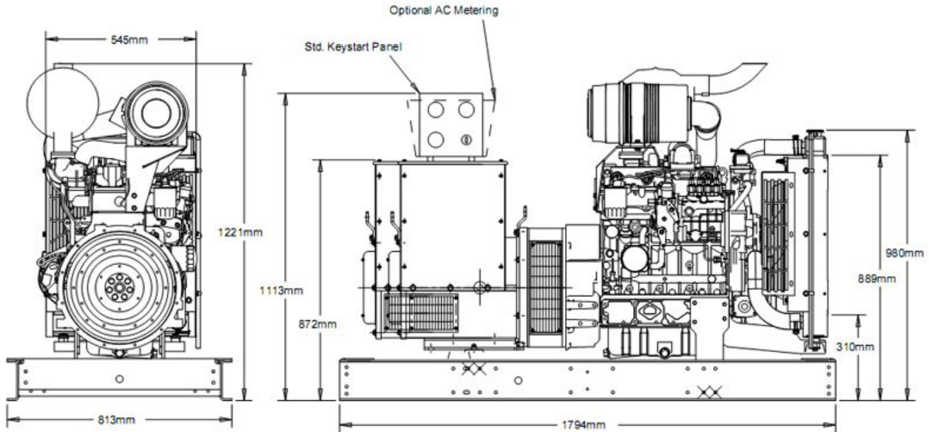
KUBOTA V3300T WITH UCI 224 C / D / E
